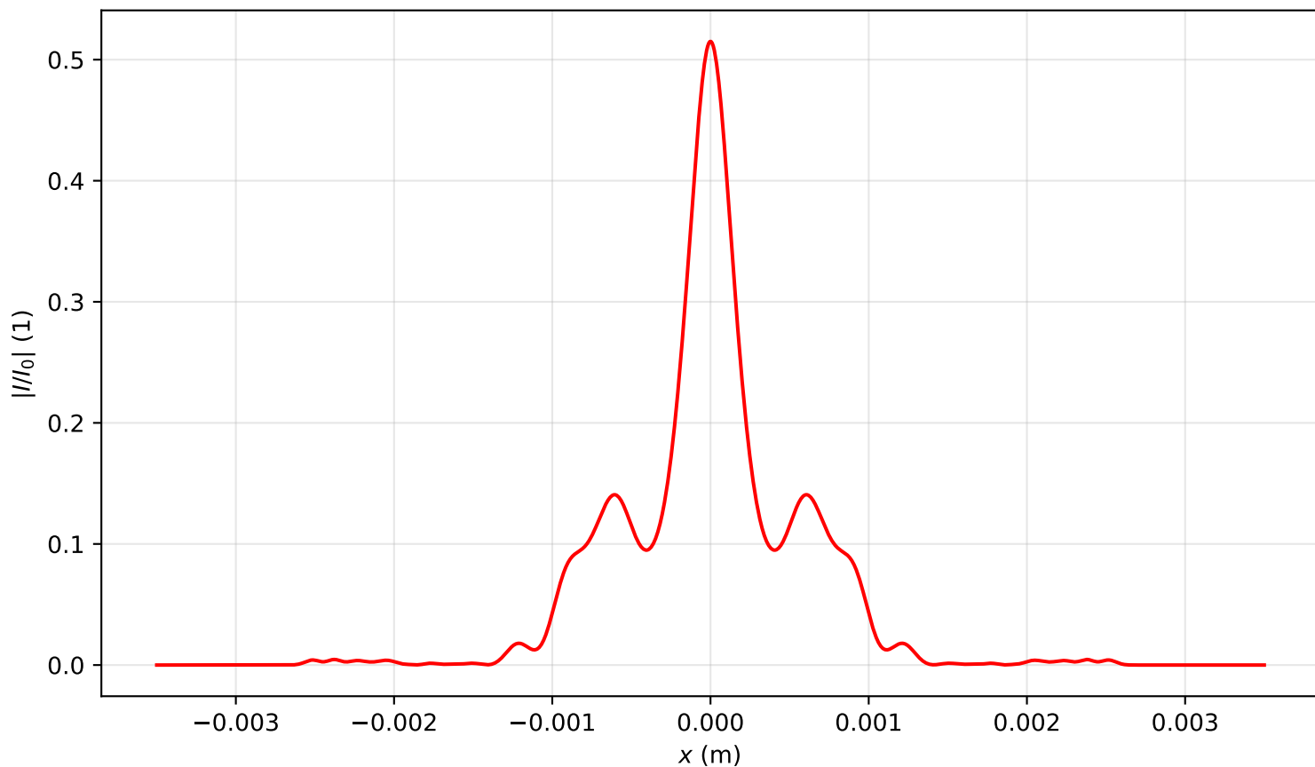
Intensity profile I(x, y = 0, z = 1.672)/I_0 , P_{in}=7.5P_{cr} , artificial time
